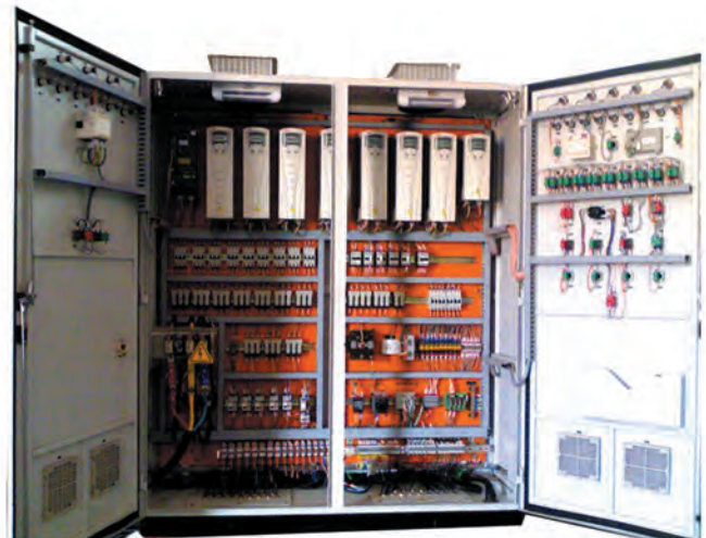
WALLMOUNTING VFD CONTROL PANEL
